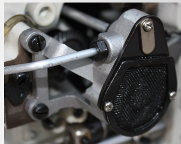
Auto lubrication from sump with oil pump
