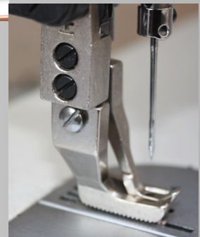
High lift to 16mm With knee press Extra feet available, piping, half foot, etc.
